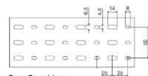
Base Punching Width 80/100/120
