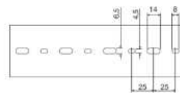
Base Punching Width 25/40/60
