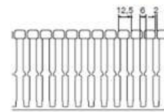
Side Stamping Height 80mm
