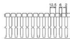
Side Stamping Height 60mm
