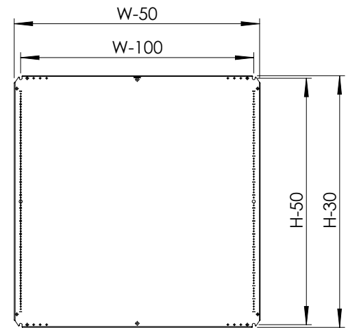
Mounting plate
