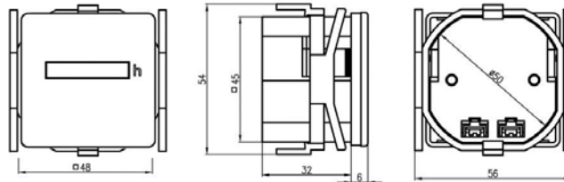
Panel Mount
