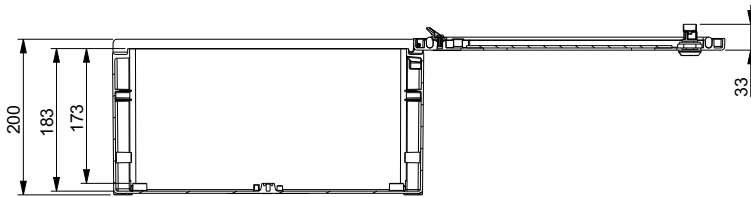
Section A
