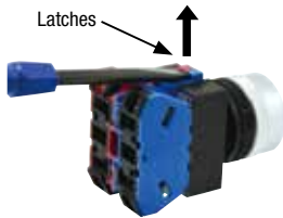
Latches
